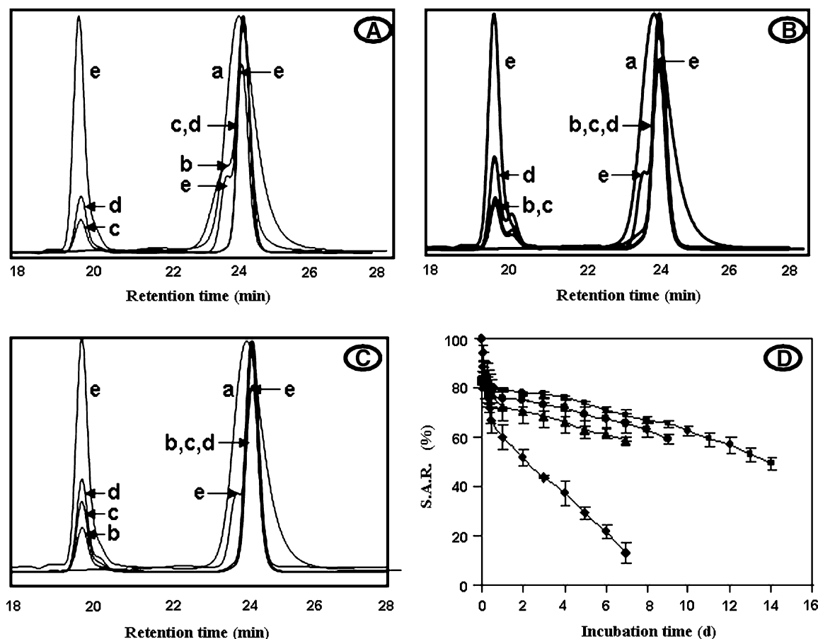
Fig. 5. (A–C) HPLC peaks of native lysozyme in 50 mM, pH 7.4 PBS (a), lysozyme extracted from fiber samples F1, F2 and F3 with protein loadings of 1.0% (A), 3.0% (B) and 5.0% (C) after incubation for 1 day (b), 1 week (c), 2 weeks (d), and free lysozyme after incubation with MC/PDLLA fibers for 2 weeks (e). (D) Specific bioactivity retention (S.A.R.) of native lysozyme (◆) and lysozyme extracted from the fiber samples F1 (■), F2 (●) and F3 (▲) during incubation ( n = 3 ).
