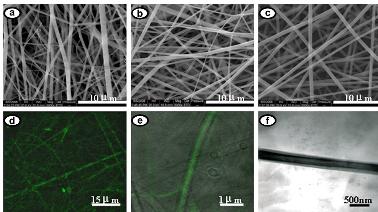
Fig. 1. Fiber morphologies and inner structures of lyz-MC/PDLLA composite fibers. SEM images of fiber samples F1, F2 and F3 prepared from emulsions with weight ratios of proteins to polymers of 1.0% (a), 3.0% (b) and 5.0% (c). Overview LCSM image of fiber sample F1 (d); LCSM (e) and TEM images (f) of a segment of fiber sample F1.
