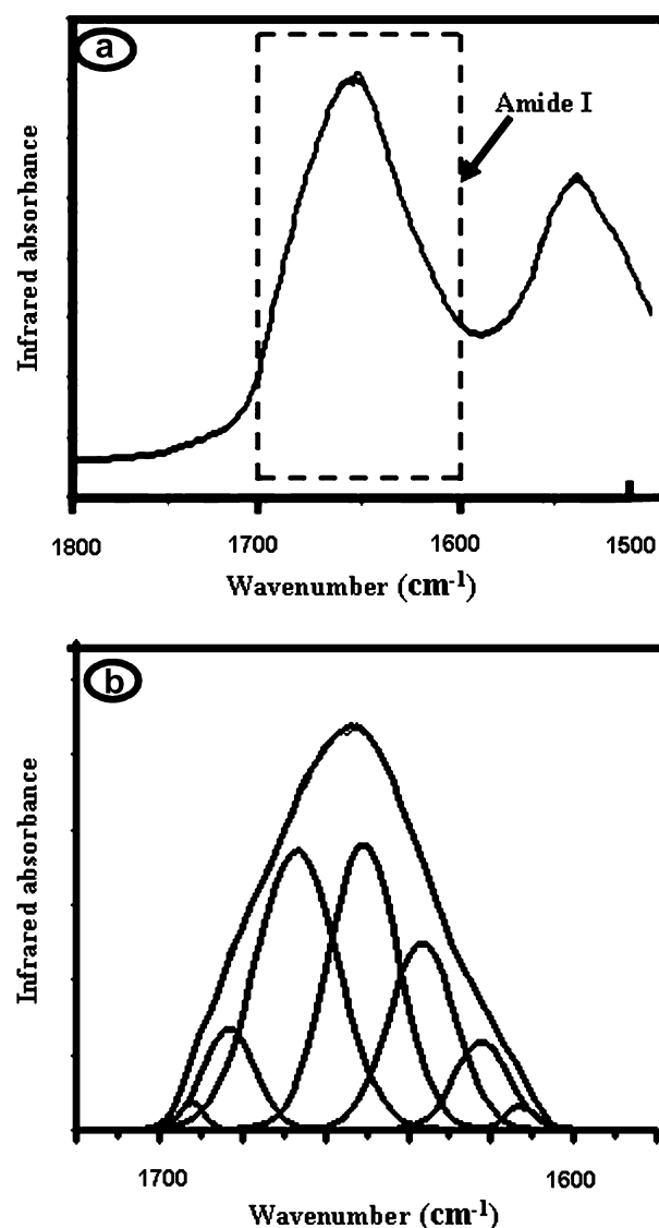
Fig. 3. Amide I region (a) and Gaussian curve-fitting Amide I region (b) of FTIR spectrum of native lysozyme in 50 mM, pH 7.4 PBS.
