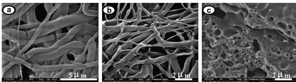
Fig. 6. SEM morphologies of lyz-MC/PDLLA fibers with lysozyme loading of 3.0% after incubated for 2 (a), 4 (b) and 8 (c) weeks in 50 mM pH 7.4 PBS at 37 °C.
